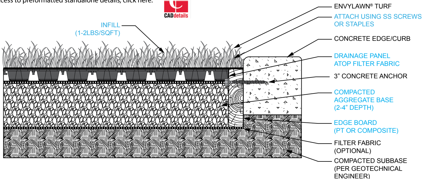
1 ENVYLAWN PET TURF - BOARD AND CURB - DETAIL SCALE: NONE
