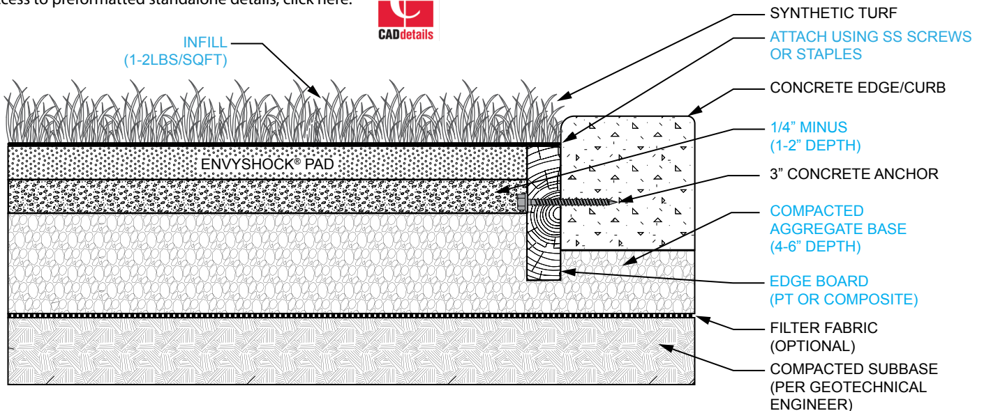
1 ENVYLAWN PLAYGROUND - BOARD AND CURB - DETAIL SCALE: NONE
