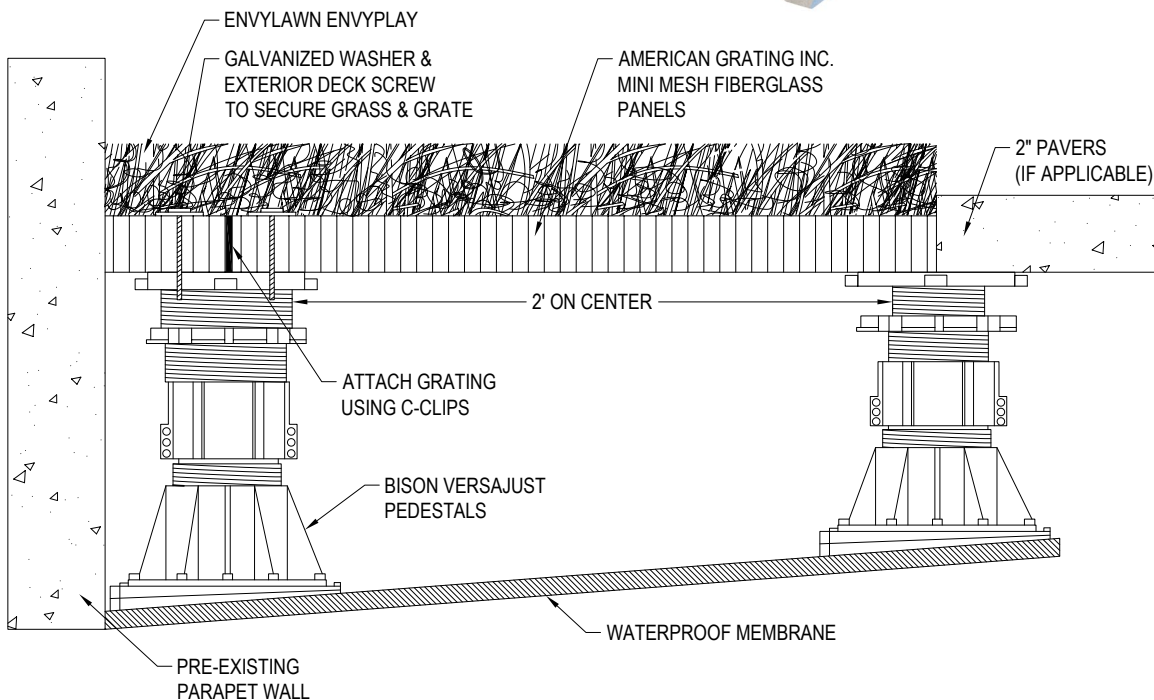
1 ENVLAWN ROOF DECK OVER PEDESTALS - DETAIL SCALE: NONE
